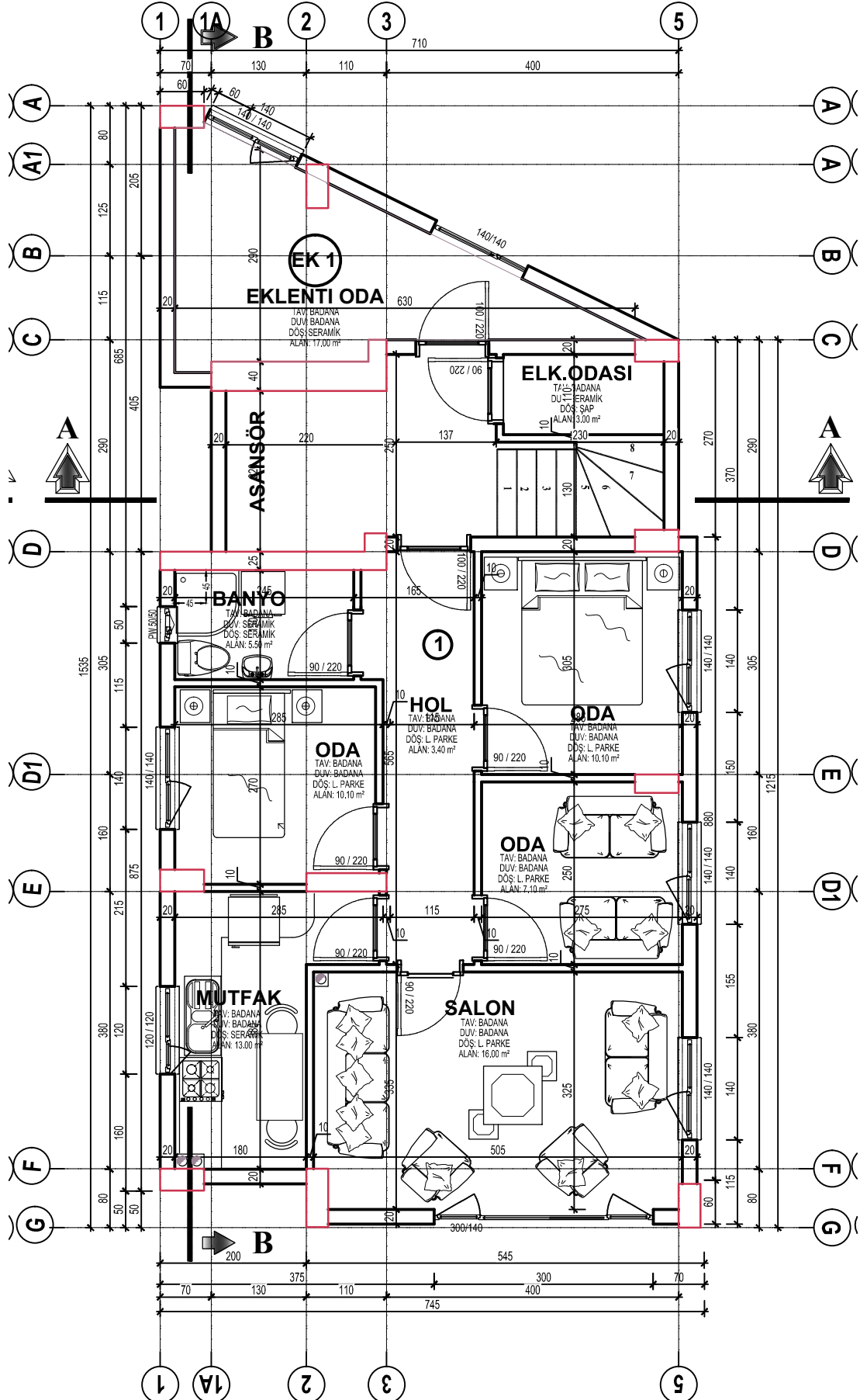
TADİLATLI 3. BODRUM KAT PLANI Ö:1/50
